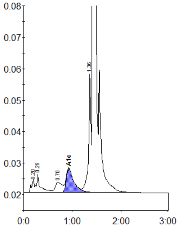
Peak table - ID: 10678662
